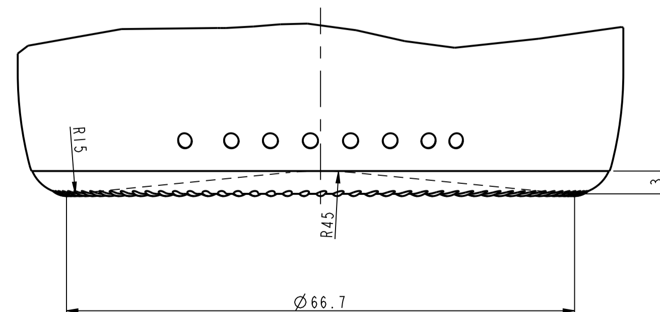
PUSH-UP CONSTRUCTION SCALE 2/1
